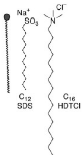
Surfactant Monomers
